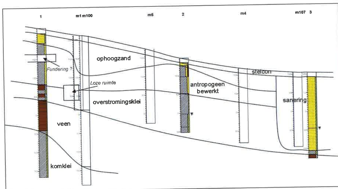
Figuur 6: Oost-west profiel.
