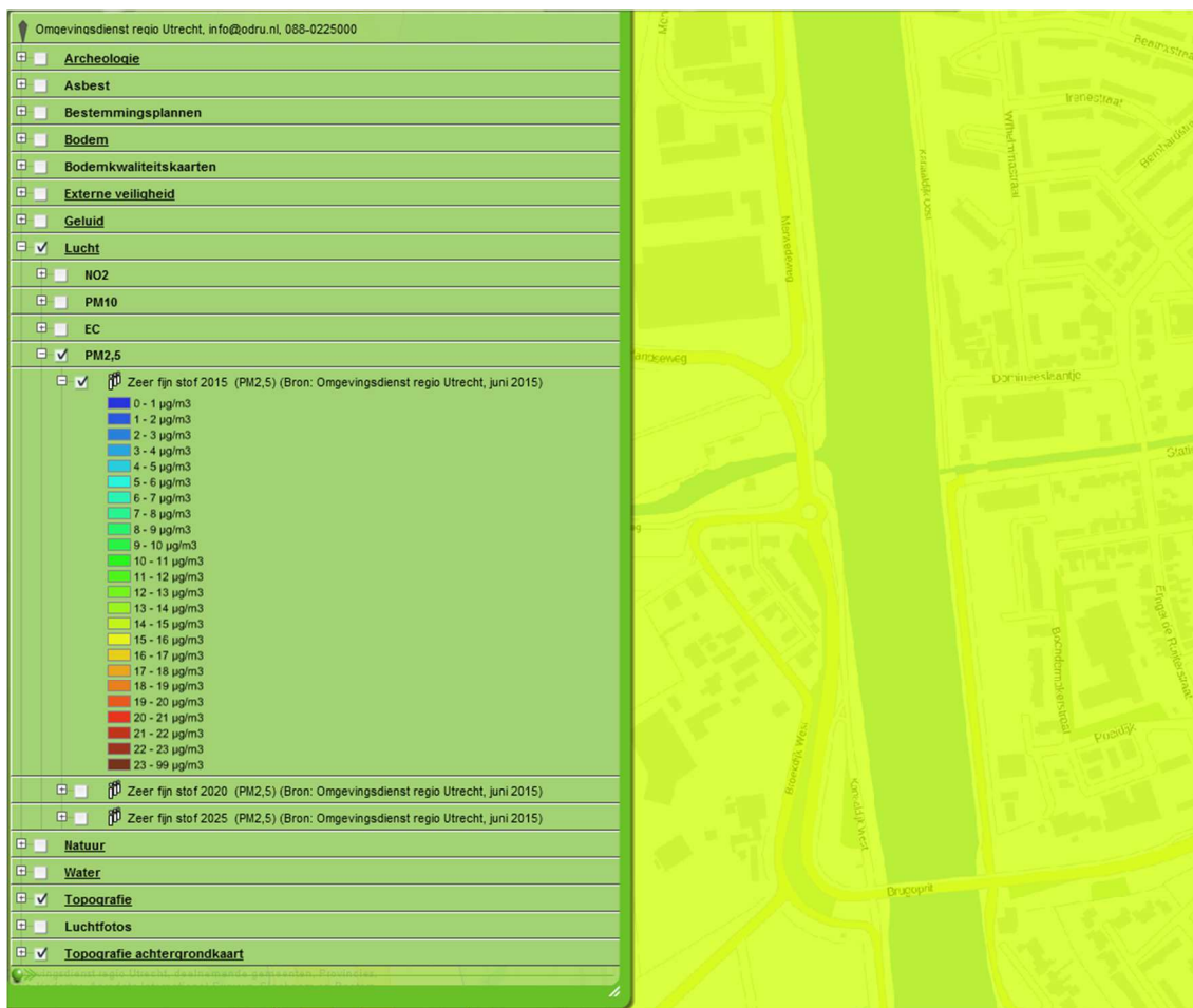
PM 2.5 , 2015
