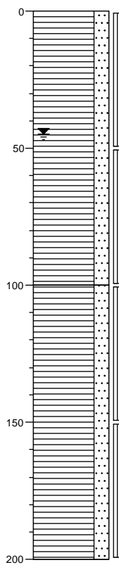
Boring: 01
