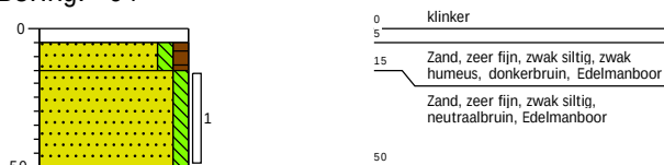
Boring: 04
