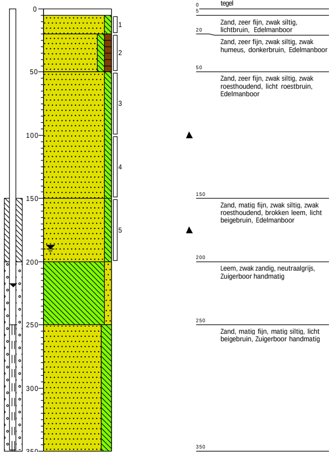
Boring: 01
