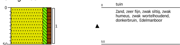
Boring: 05
