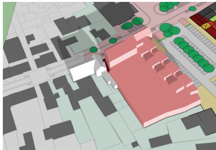
11:00 - 21 december
