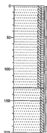
Boring: 5
