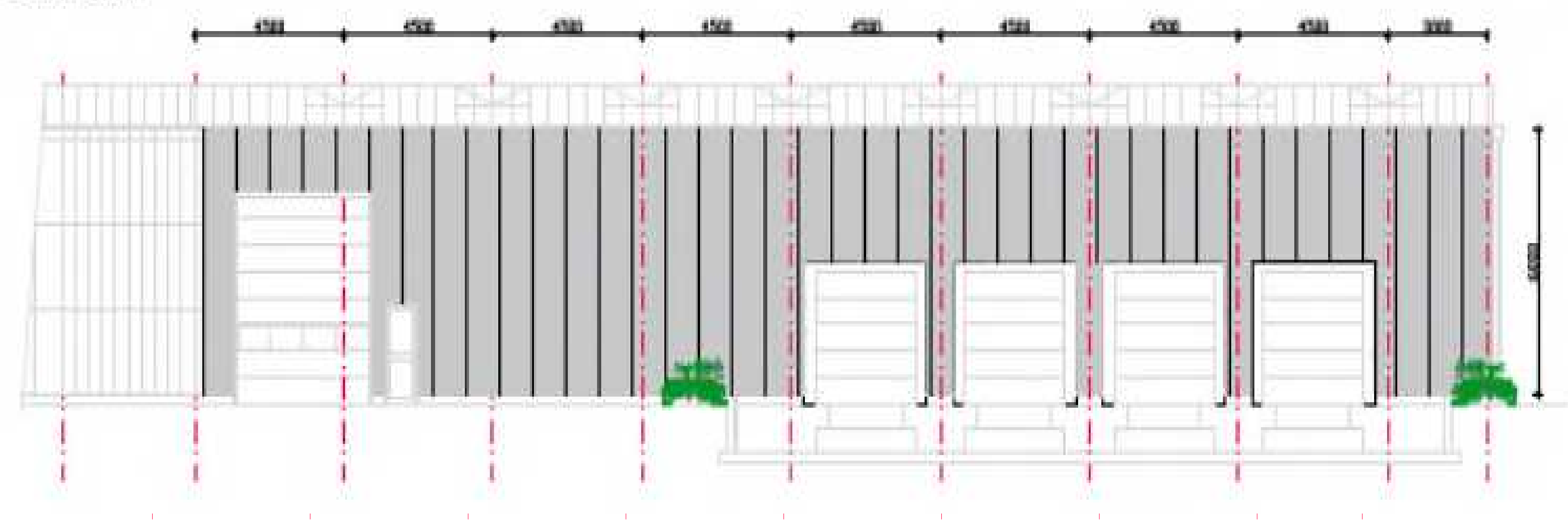
Aanzicht as 12 school 1000
