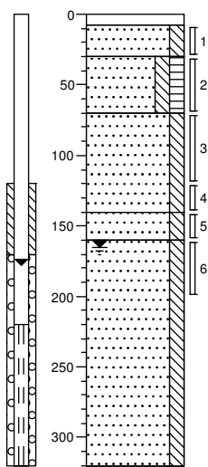
Boring: 01
