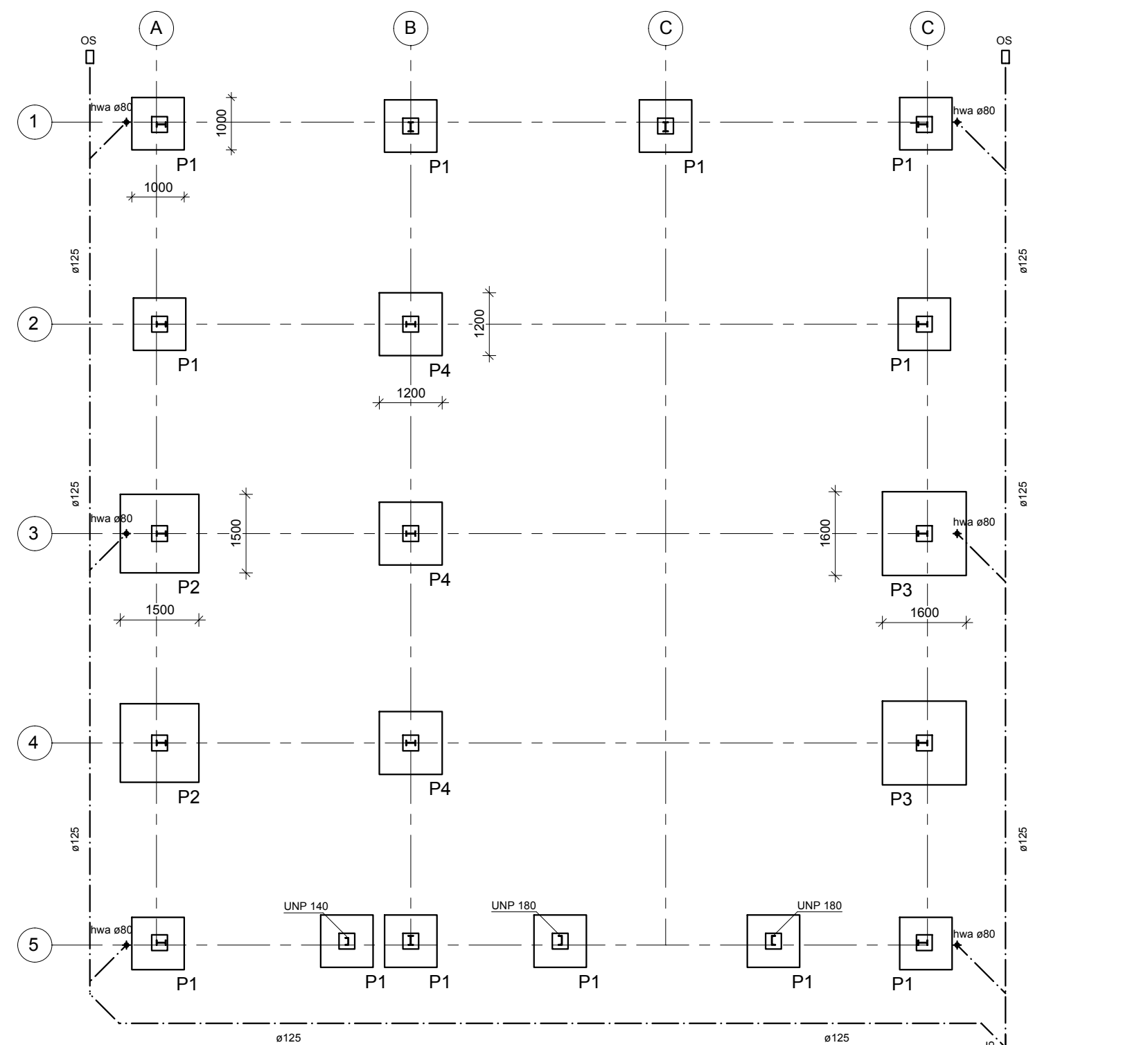
Fundering
