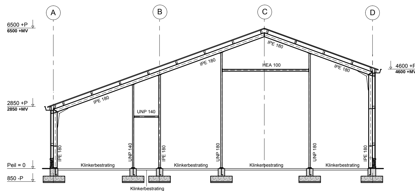
Gevel as 1
