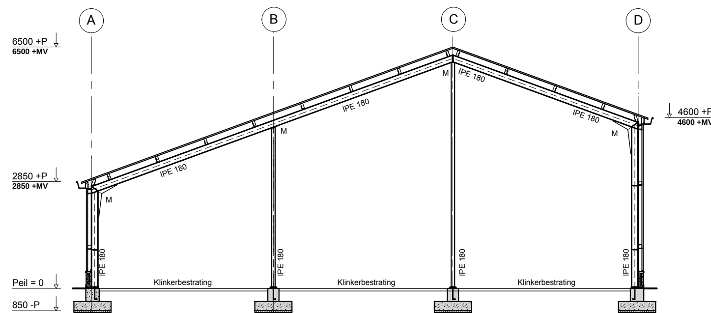
Gevel as 1
