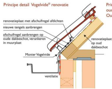
Principe detail Vogelvide® renovatie
