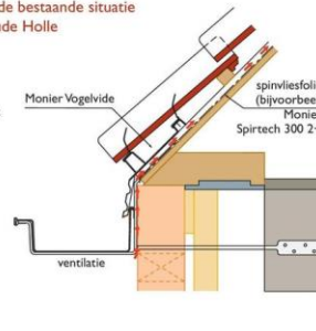
Principe detail Vogelvide® met gootplank
