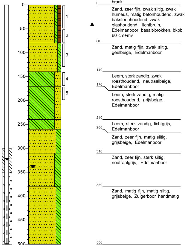
Boring: 01
