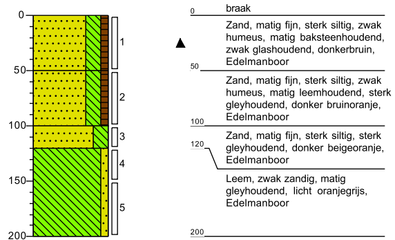
Boring: 03
