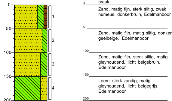
Boring: 02
