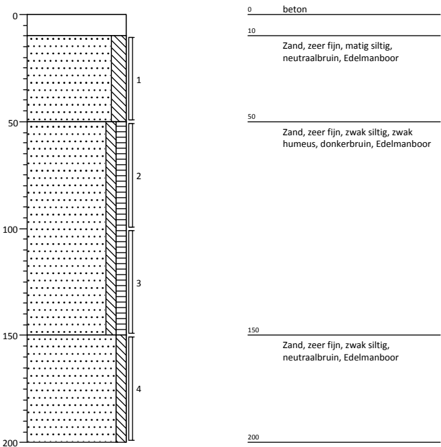
Boring: 03
