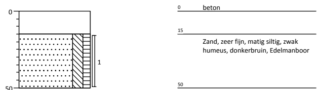
Boring: 08
