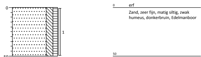
Boring: 09
