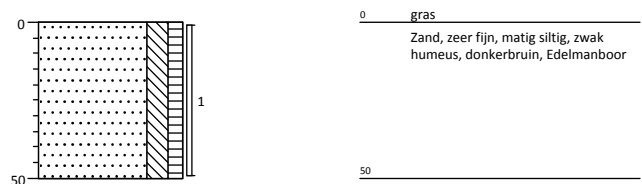
Boring: 06
