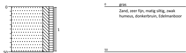
Boring: 07
