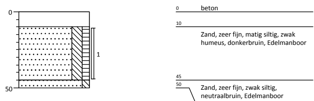
Boring: 10
