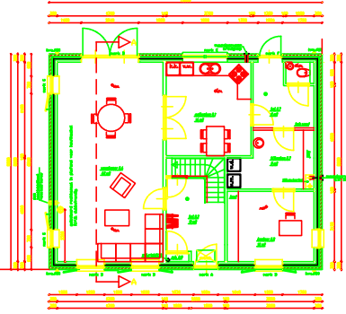
BEGANE-GROND
