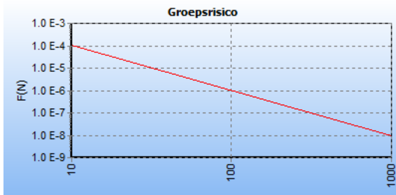
Figuur 2.1 FN-Curve
