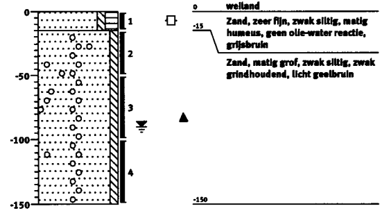
Boring: 22
