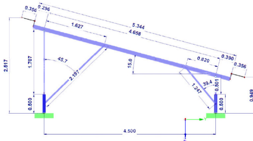
Figure 1 – projected mounting structure (EA)
