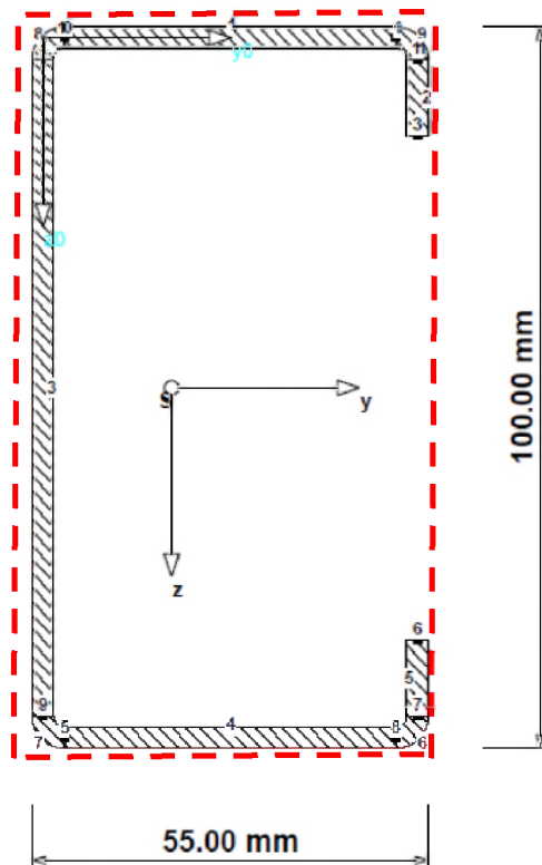
Figure 5 – Area of skin fiction of C100x55 pile
