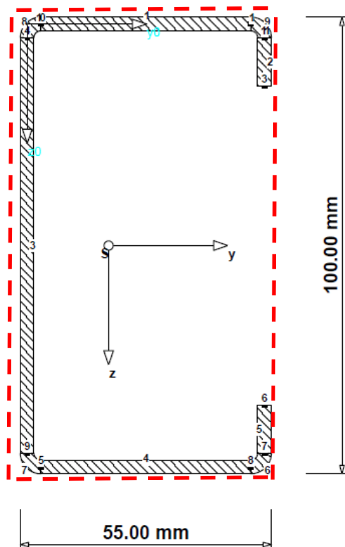
Figure 5 – Area of skin fiction of C100x55 pile
