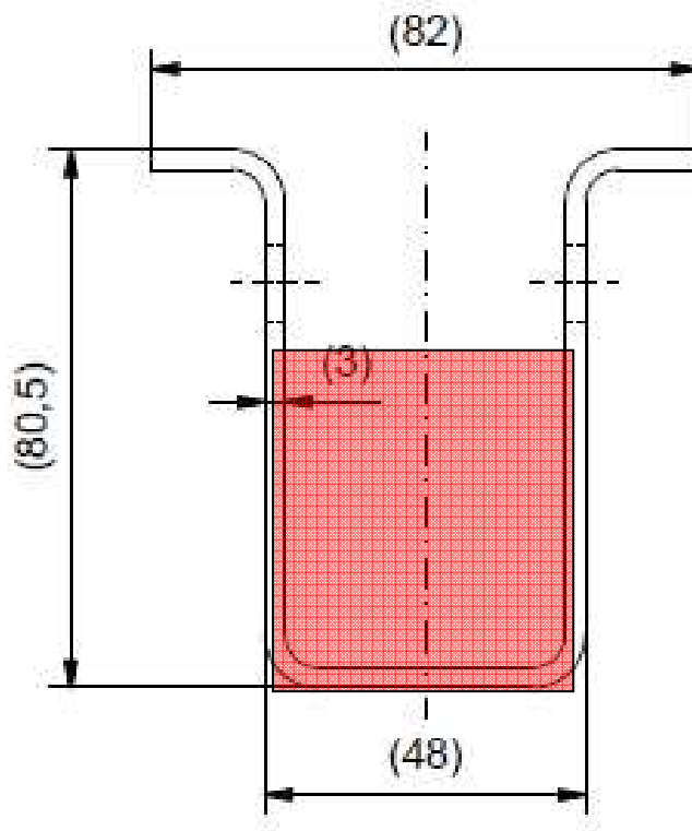
Figure 8 – Area of tip of Hat pile
