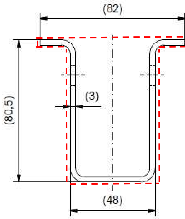
Figure 6 – Area of the skin fiction of Hat pile
