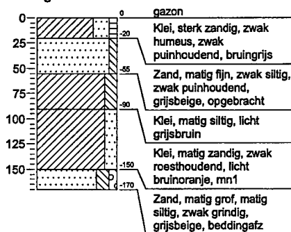
Boring: 28
