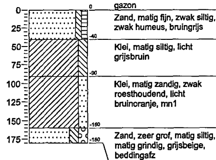
Boring: 26
