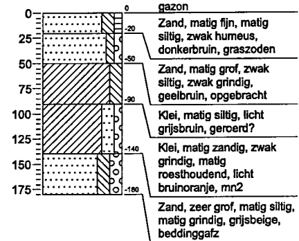
Boring: 12
