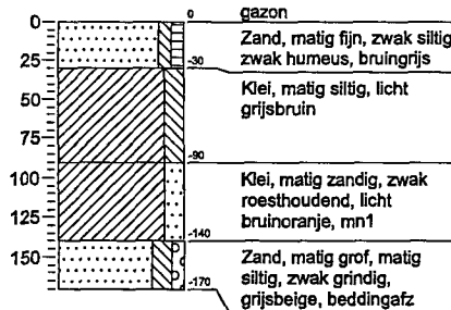
Boring: 25
