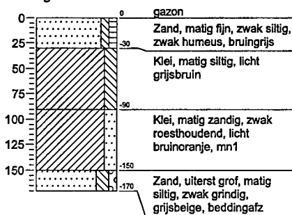
Boring: 31
