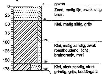
Boring: 33
