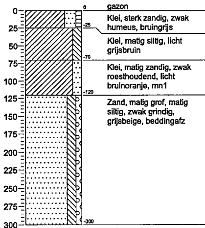
Boring: 35
