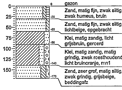
Boring: 50
