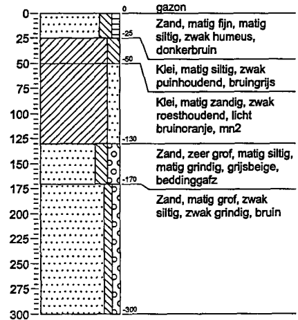
Boring: 21
