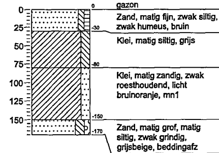
Boring: 27
