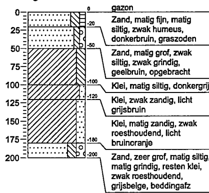
Boring: 14
