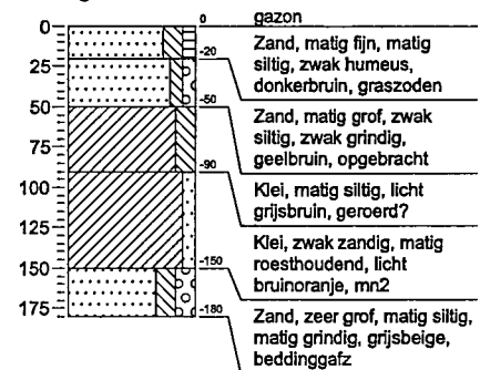
Boring: 6
