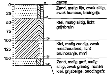
Boring: 24
