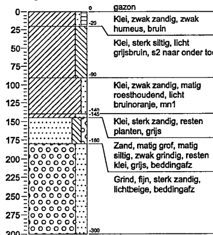
Boring: 17
