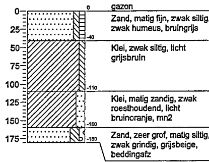
Boring: 47
