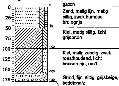
Boring: 29
