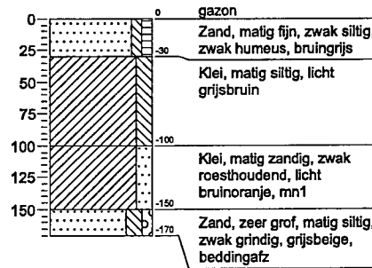
Boring: 36
