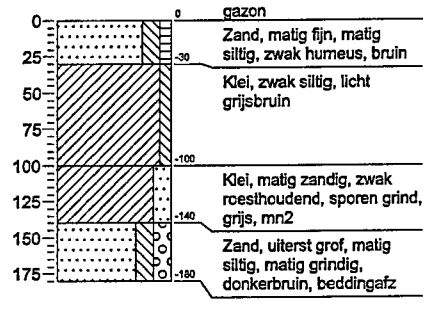
Boring: 48
