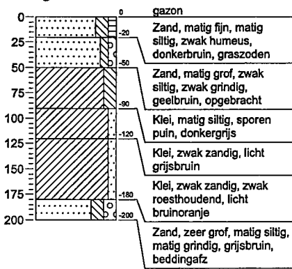
Boring: 13
